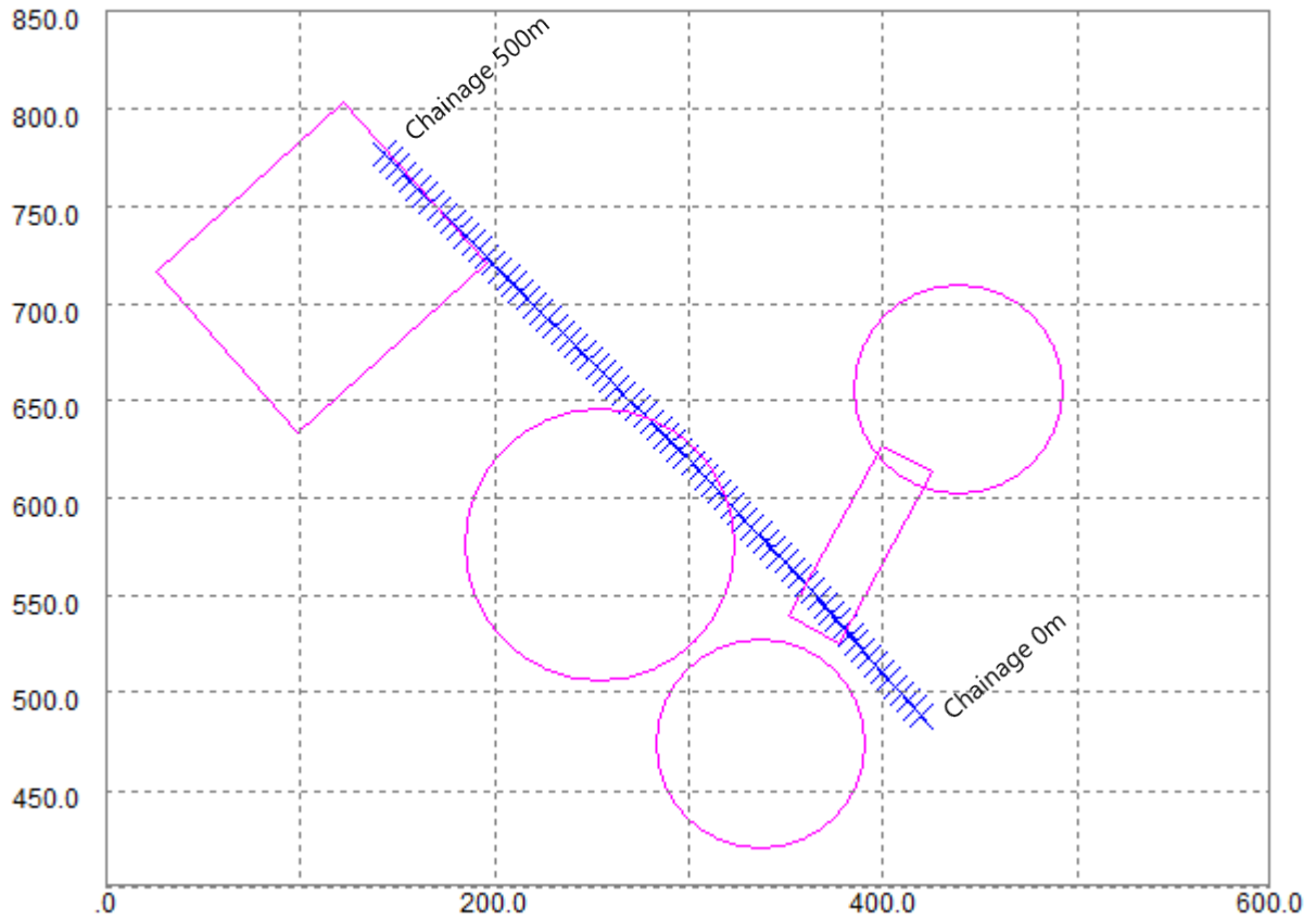
Figure 5-2 Graphical Representation of PDISP Model
